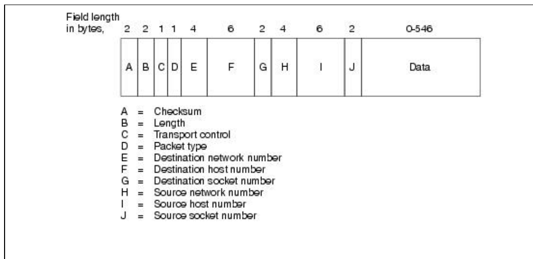
Figure: Eleven Fields Comprise an IDP Packet
