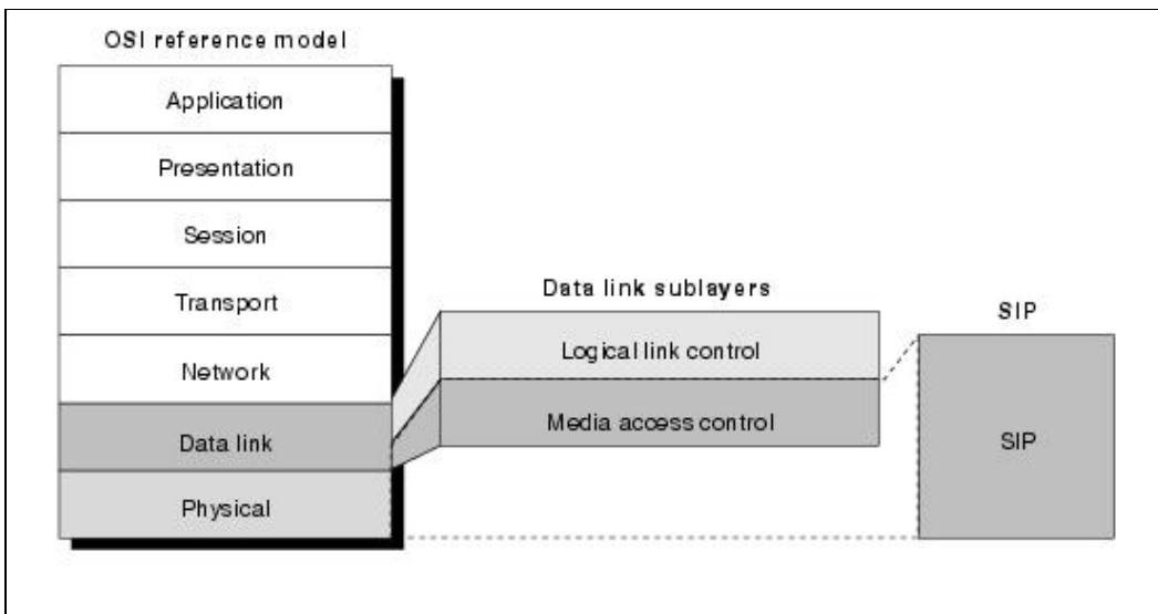
Figure: SIP Provides Services Associated with the Physical and Data Link Layers of the OSI Model SIP Level
