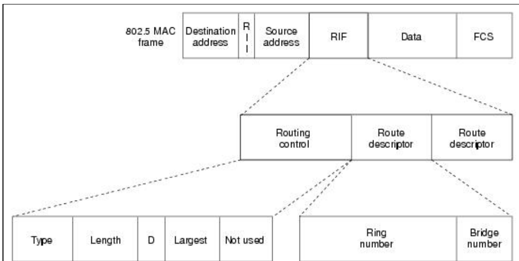
Figure: An IEEE 802.5 RIF Is Present in Frames Destined for Other LANs
