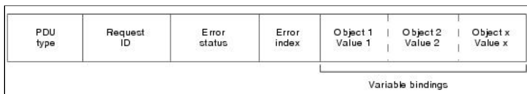
Figure: SNMPv2 Get, GetNext, Inform, Response, Set, and Trap PDUs Contain the Same Fields
