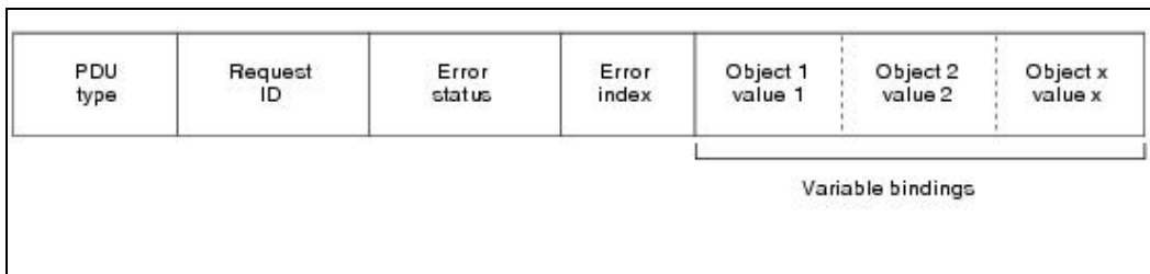
Figure: SNMPv1 Get, GetNext, Response, and Set PDUs Contain the Same Fields
