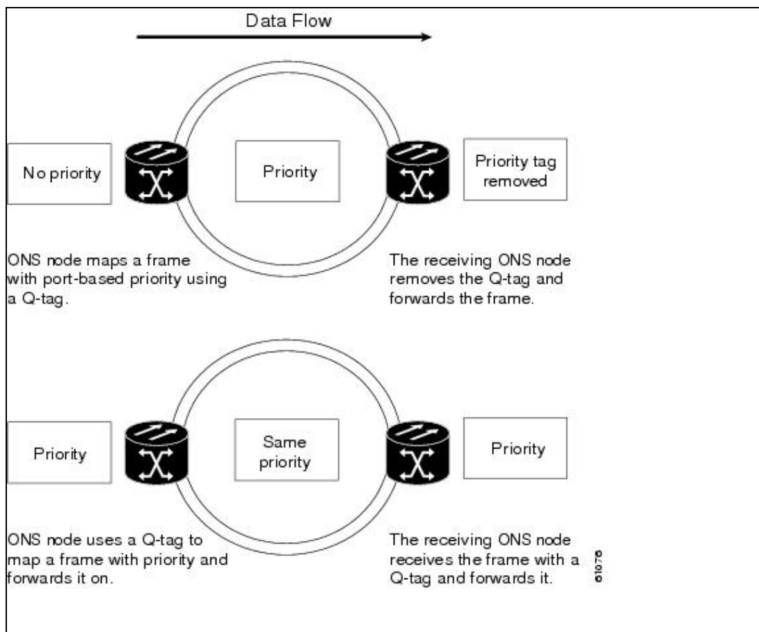
Figure 25-16: Priority Queuing Process
