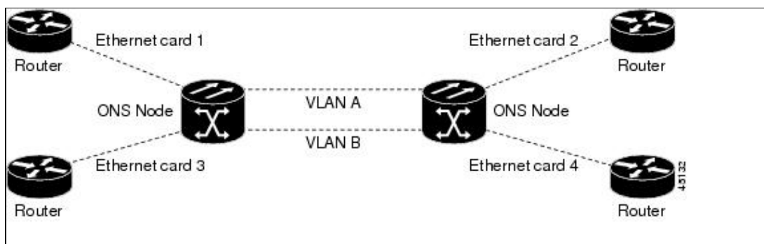
Figure 25-12: Single-Card EtherSwitch Configuration
