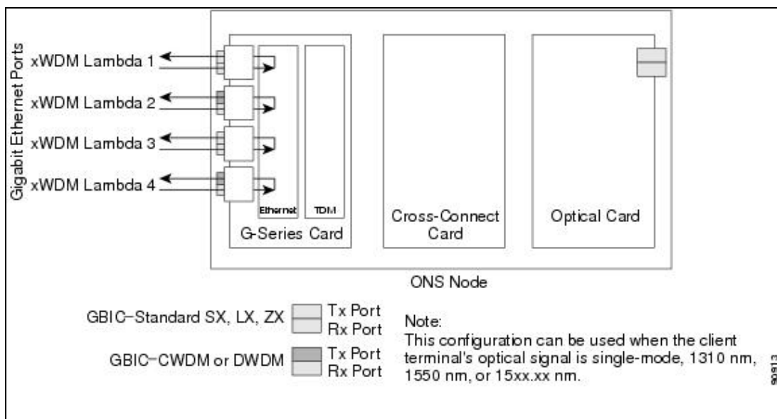
Figure 25-9: One-Port Bidirectional Transponder Mode
