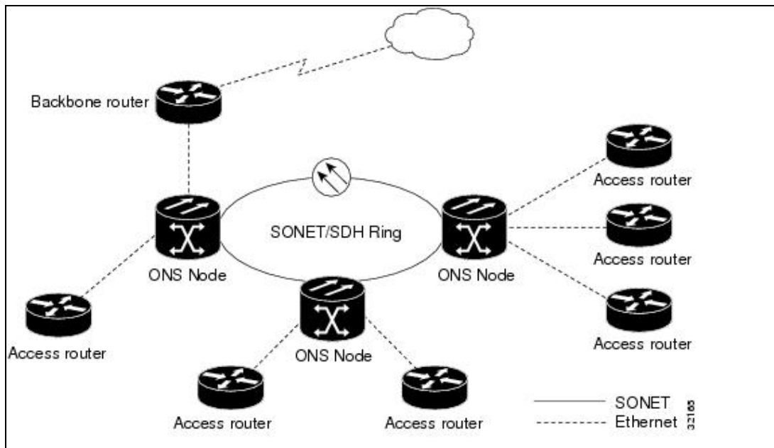
Figure 25-21: Shared Packet Ring Ethernet Circuit
