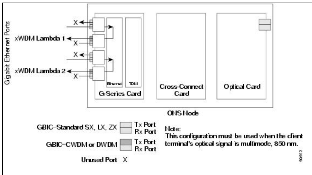
Figure 25-10: Two-Port Unidirectional Transponder
