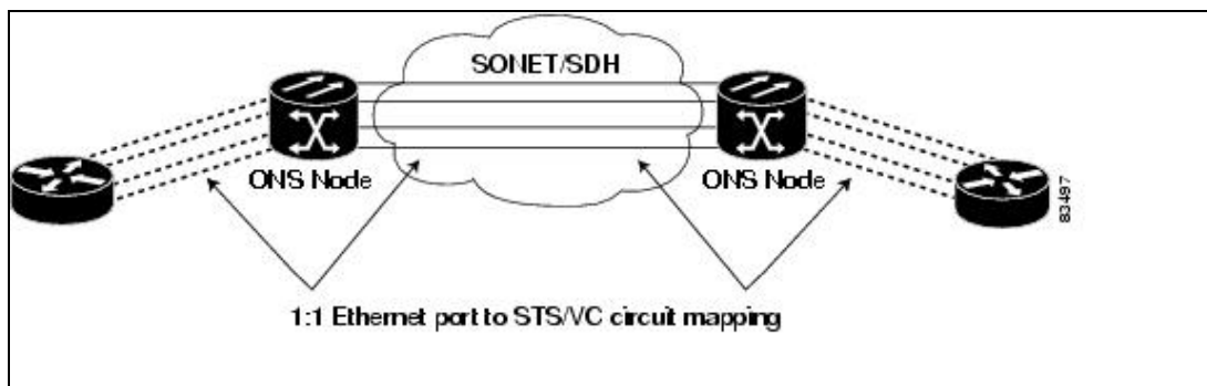
Figure 25-13: E-Series Mapping Ethernet Ports to STS/VC Circuits
