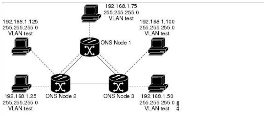
Figure 25-22: Hub-and-Spoke Ethernet Circuit
