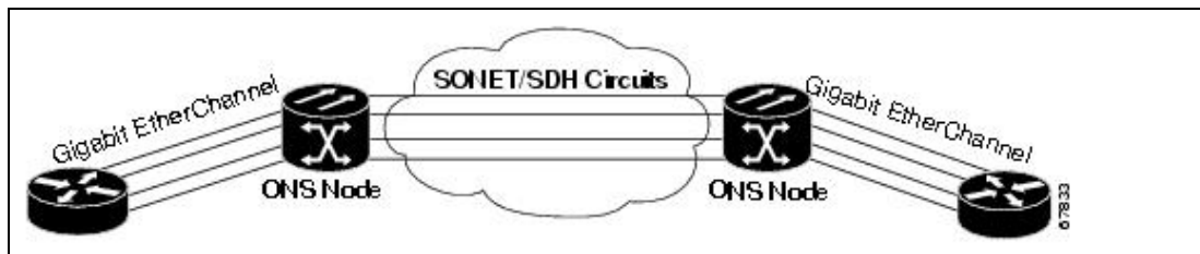
Figure 25-2: G-Series Gigabit EtherChannel (GEC) Support
