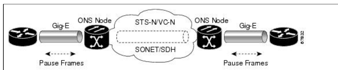
Figure 25-1: Data Traffic on a G-Series Point-to-Point Circuit
