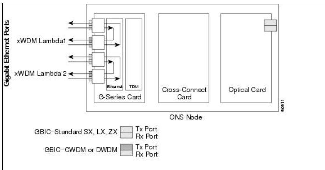
Figure 25-8: G-Series Card in Transponder Mode (Two-Port Bidirectional)
