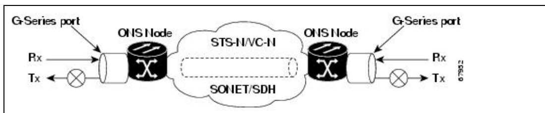
Figure 25-3: End-to-End Ethernet Link Integrity Support
