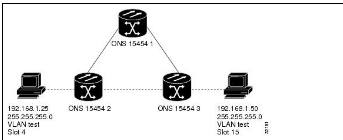
Figure 25-20: Single-Card EtherSwitch or Port-Mapped Point-to-Point Circuit
