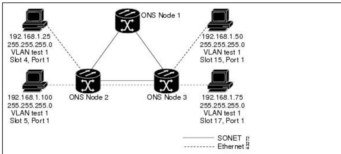
Figure 25-19: Multicard EtherSwitch Point-to-Point Circuit
