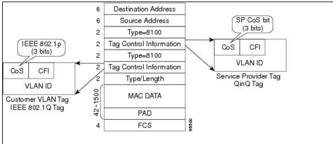
Figure 14-6: QinQ
