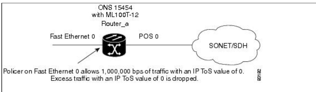
Figure 14-8: ML-Series Policing Example
