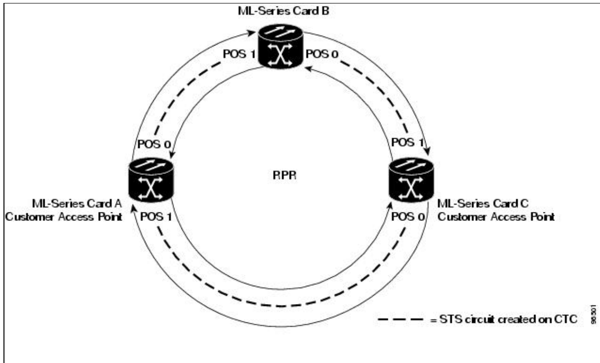
Figure 14-9: ML-Series CoS Example
