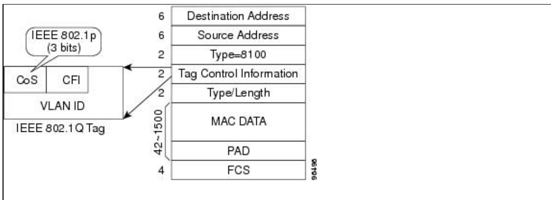
Figure 14-2: Ethernet Frame and the CoS Bit (IEEE 802.1p)
