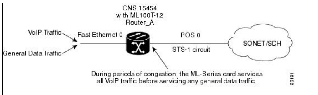
Figure 14-7: ML-Series VoIP Example
