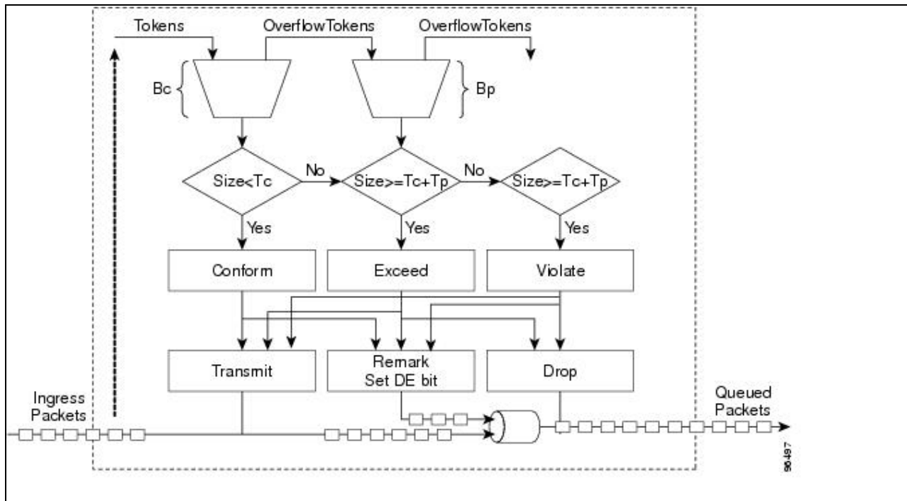
Figure 14-4: Dual Leaky Bucket Policor Model
