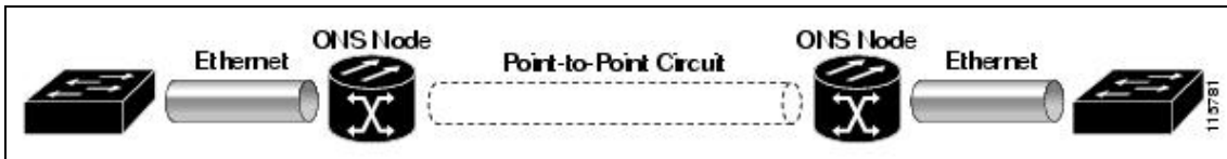
Figure 21-1: CE-1000-4 Point-to-Point Circuit
