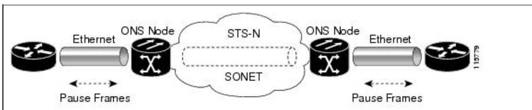
Figure 21-10: Flow Control
