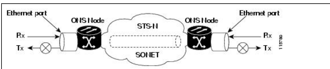
Figure 21-6: End-to-End Ethernet Link Integrity Support
