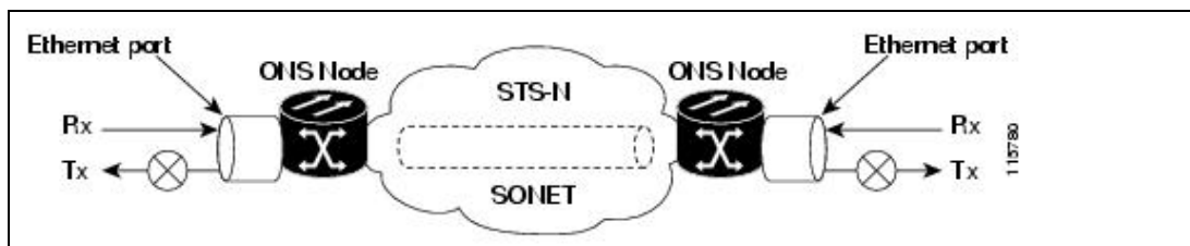
Figure 21-3: End-to-End Ethernet Link Integrity Support
