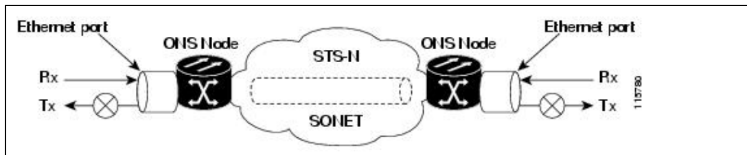
Figure 21-11: End-to-End Ethernet Link Integrity Support
