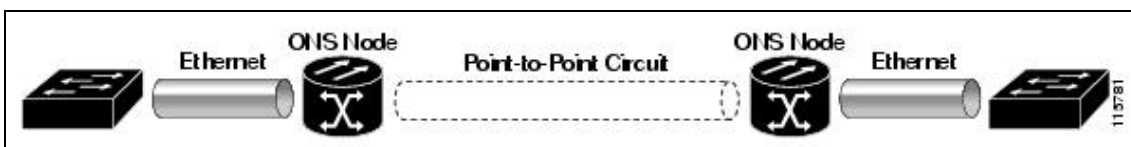
Figure 21-4: CE-100T-8 Point-to-Point Circuit
