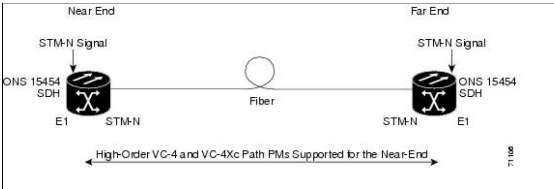
Figure 15-13: Monitored Signal Types for STM-16 and STM-64 Cards
