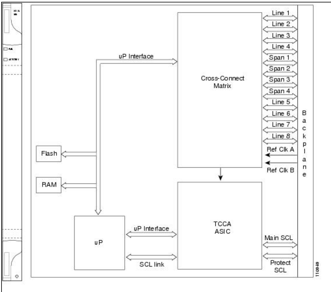
Figure 2-3: XC-VXL-10G Faceplate and Block Diagram
