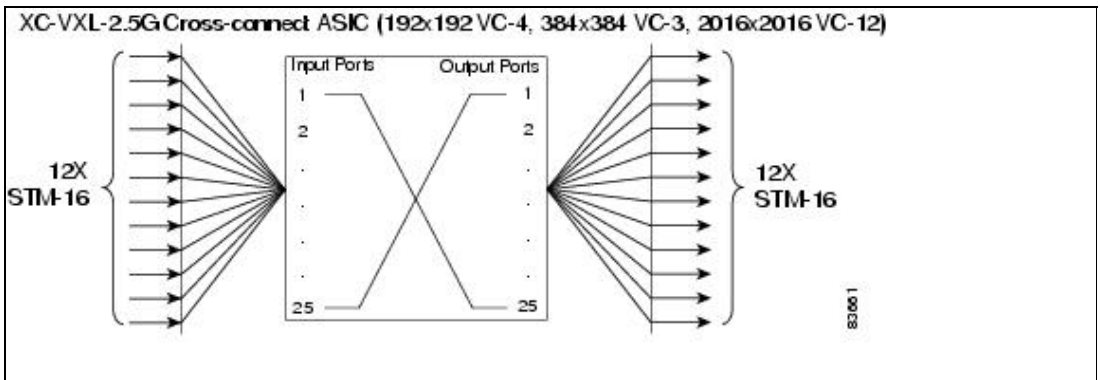
Figure 2-6: XC-VXL-2.5G Cross-Connect Matrix
