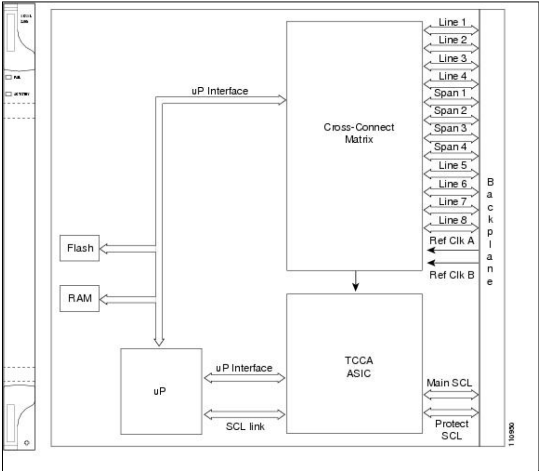
Figure 2-6 shows the XC-VXL-2.5G cross-connect matrix.
