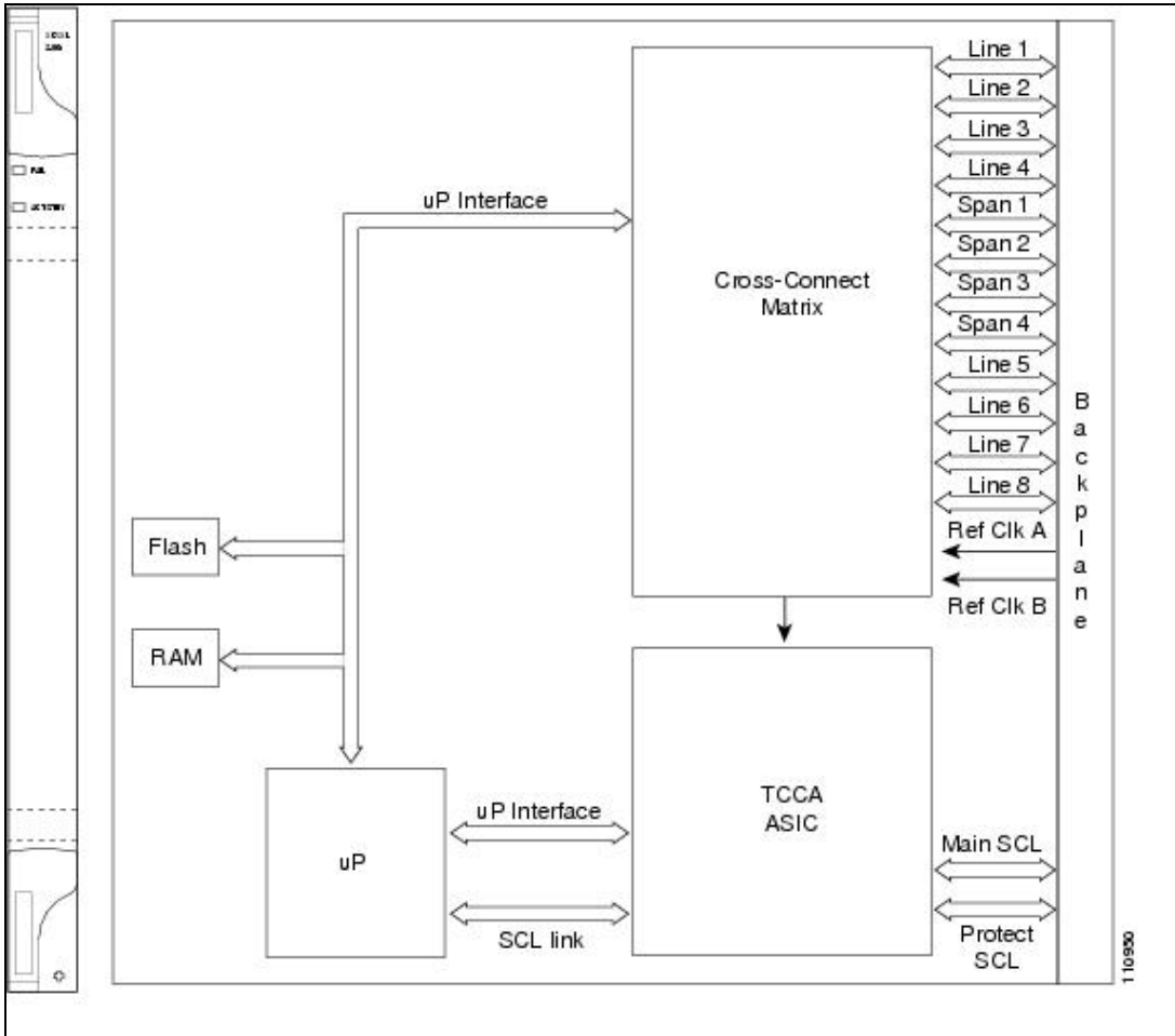
Figure 2-5: XC-VXL-2.5G Faceplate and Block Diagram
