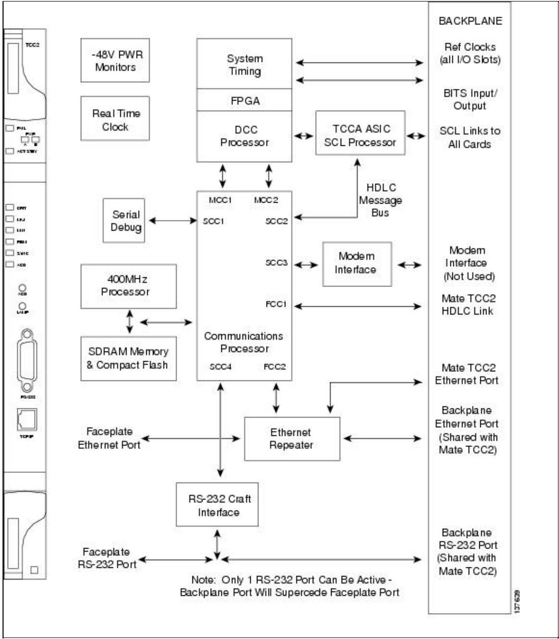
Figure 2-1: TCC2 Faceplate and Block Diagram
