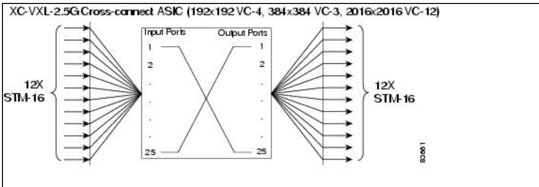
Figure 2-6: XC-VXL-2.5G Cross-Connect Matrix
