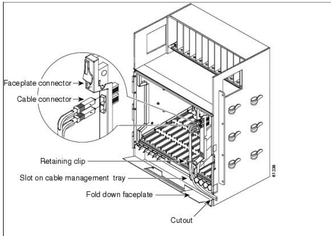
Figure 2-3: Routing Fiber-Optic Cables on the Optical-Card Faceplate
