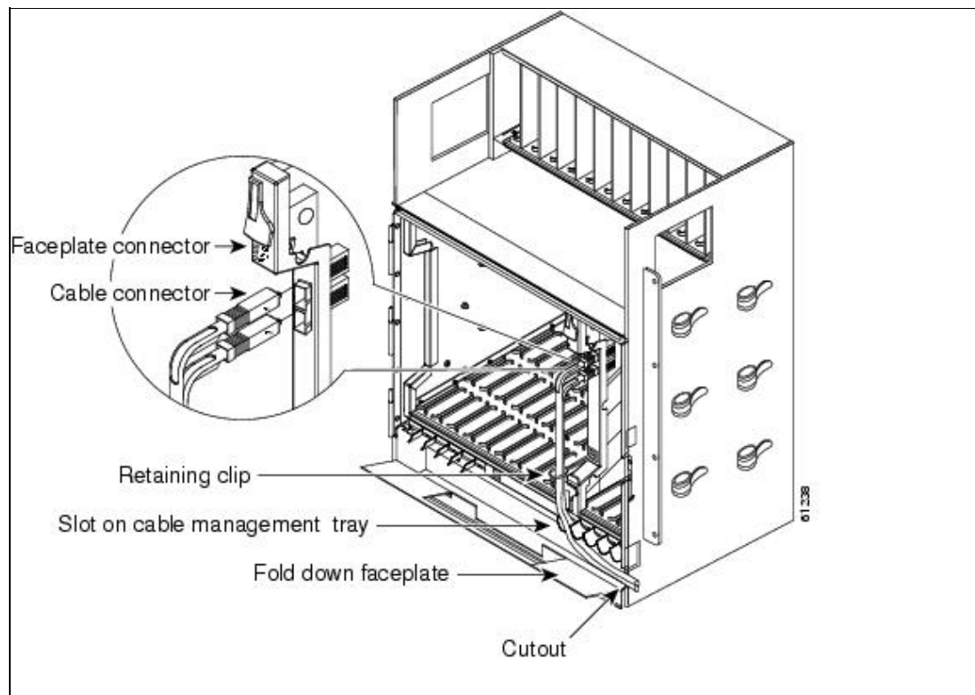
Figure 2-3: Routing Fiber-Optic Cables on the Optical-Card Faceplate
