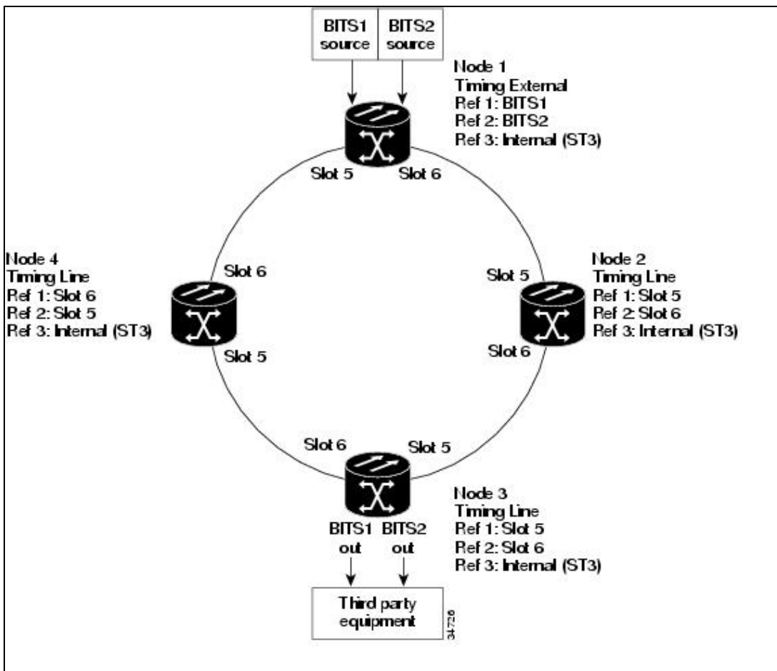
Figure 10-1: ONS 15454 Timing Example
