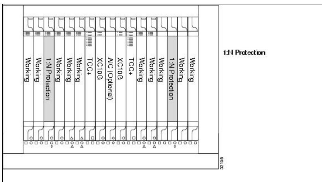
Figure 7-2: Example: ONS 15454 Cards in a 1:N Protection Configuration (SMB EIA)
