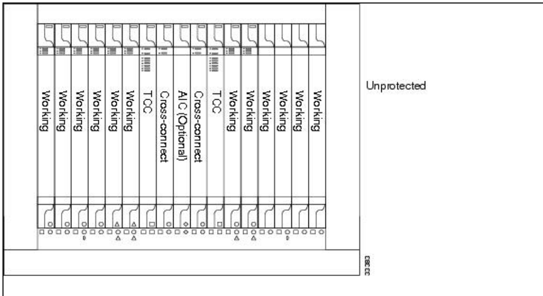
Figure 7-8: ONS 15454 in an Unprotected Configuration
