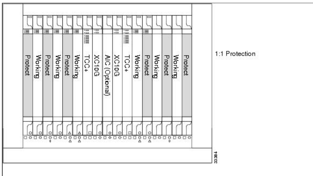
Figure 7-1: Example: ONS 15454 Cards in a 1:1 Protection Configuration (SMB EIA)
