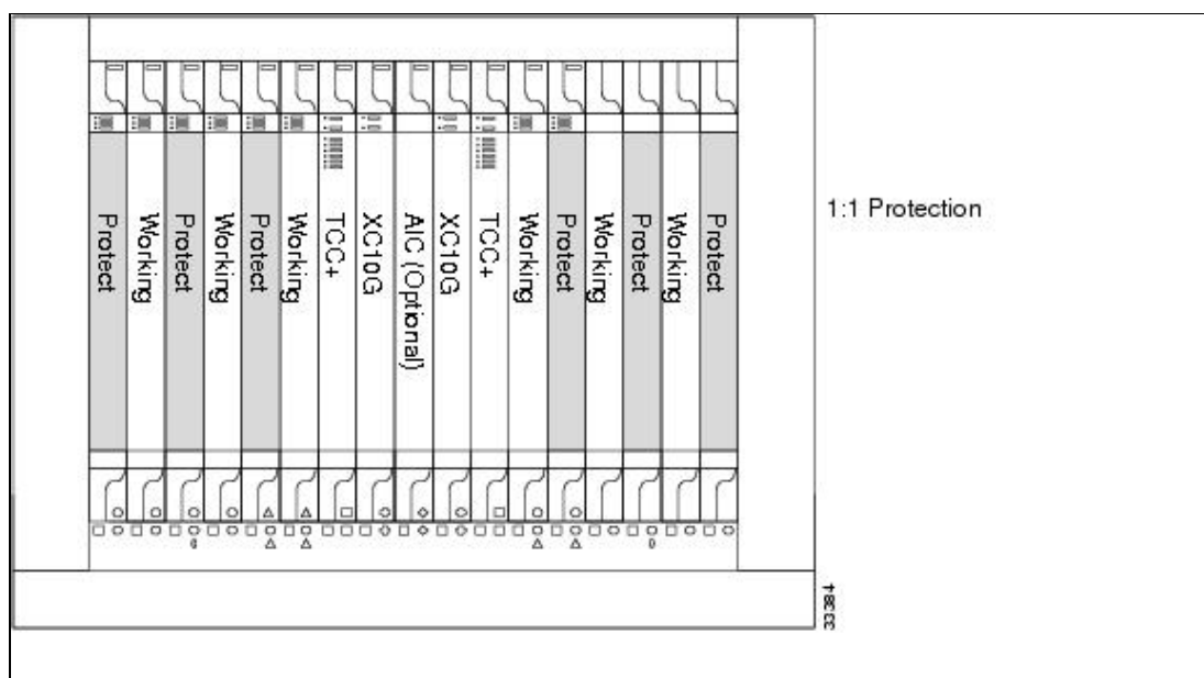
Figure 7-1: Example: ONS 15454 Cards in a 1:1 Protection Configuration (SMB EIA)
