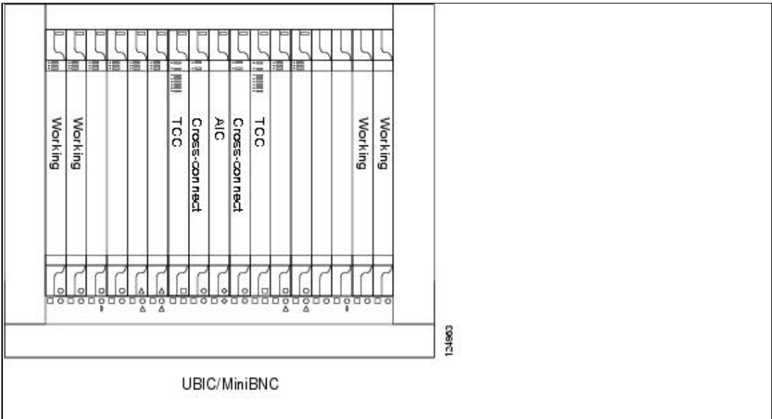
Figure 7-5 shows 1:1 low-density card protection by EIA type.
