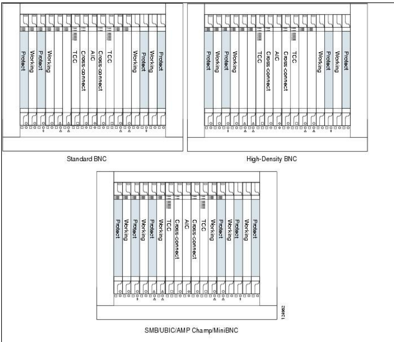
Figure 7-5: 1:1 Protection Schemes for Low-Density Electrical Cards with EIA Types
