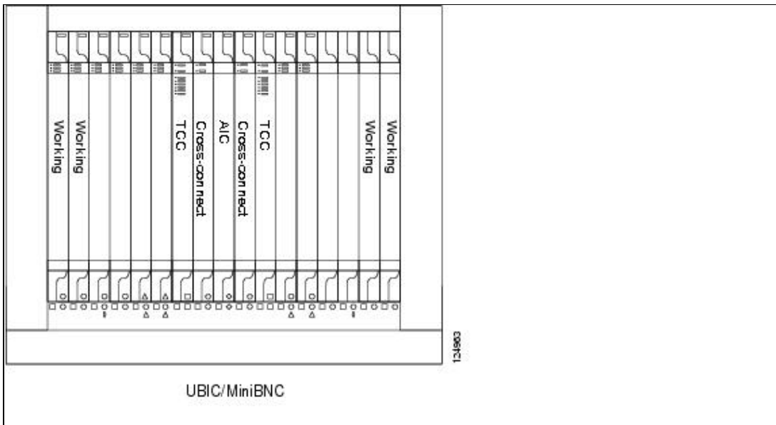
Figure 7-5 shows 1:1 low-density card protection by EIA type.
