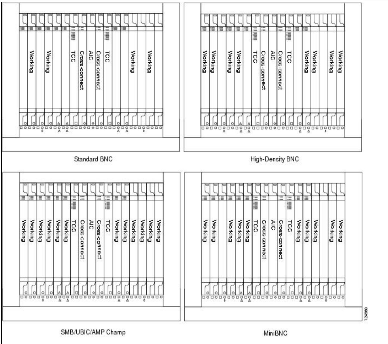
Figure 7-4 shows unprotected high-density electrical card schemes by EIA type.
