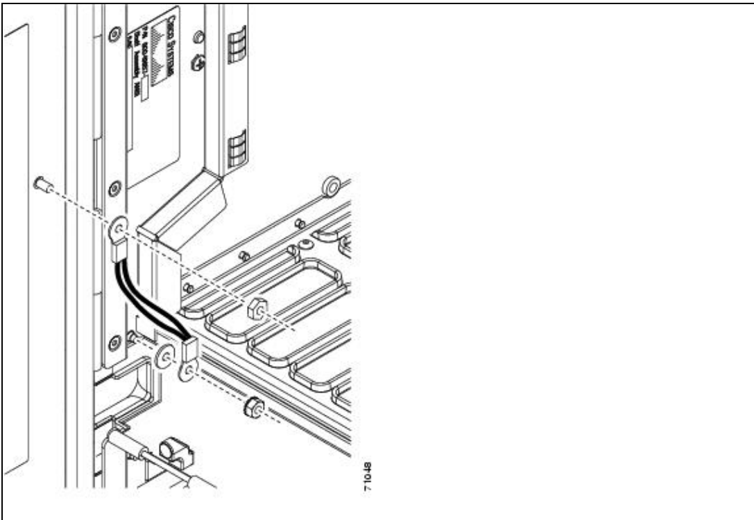
Figure 2-1: Installing the Door Ground Strap Retrofit Kit
