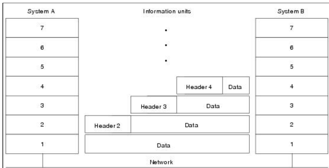
Figure: Headers and Data Can Be Encapsulated During Information Exchange
