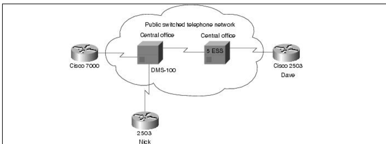
Figure: ISDN network example
