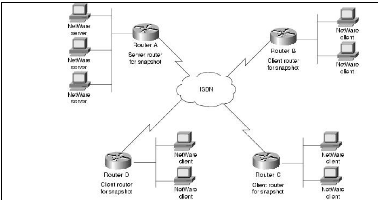
Figure: Topology of the Novell IPX network
