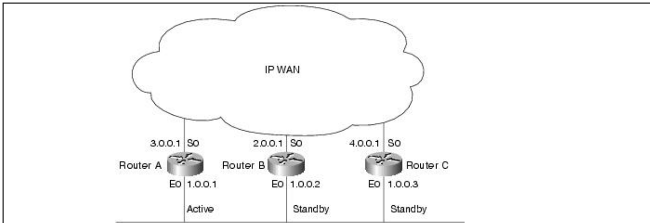
Figure: A network with tracking configured
