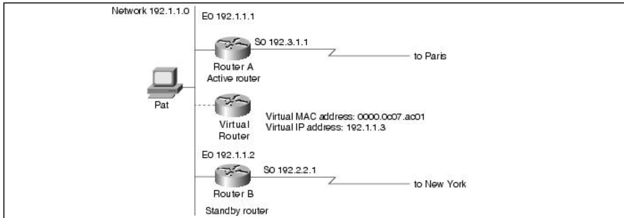
Figure: HSRP addressing on the Tokyo segment
