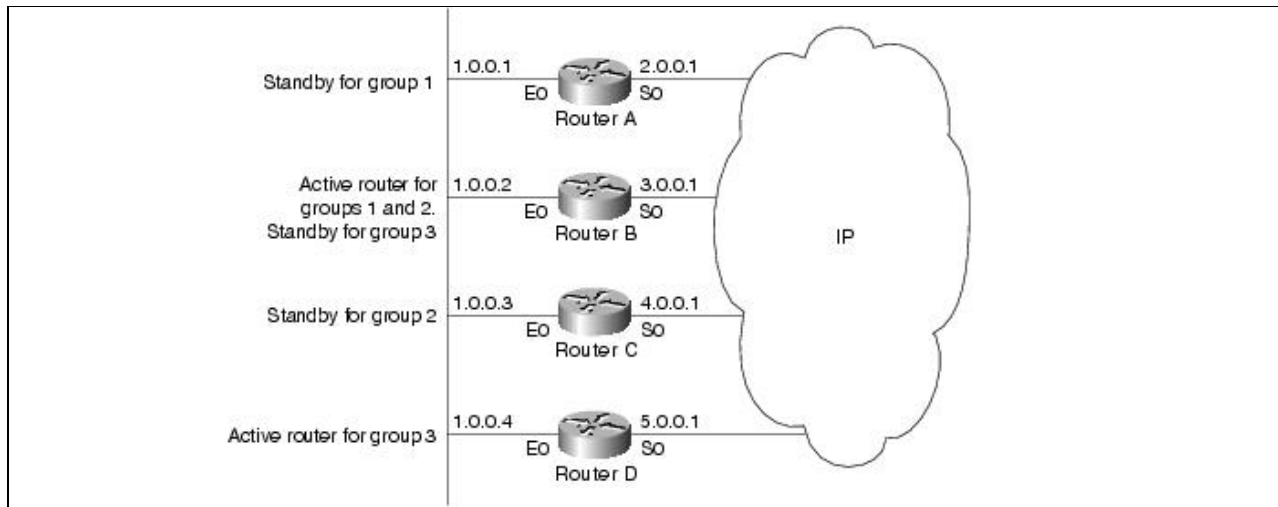
Figure: Example of hot standby groups
