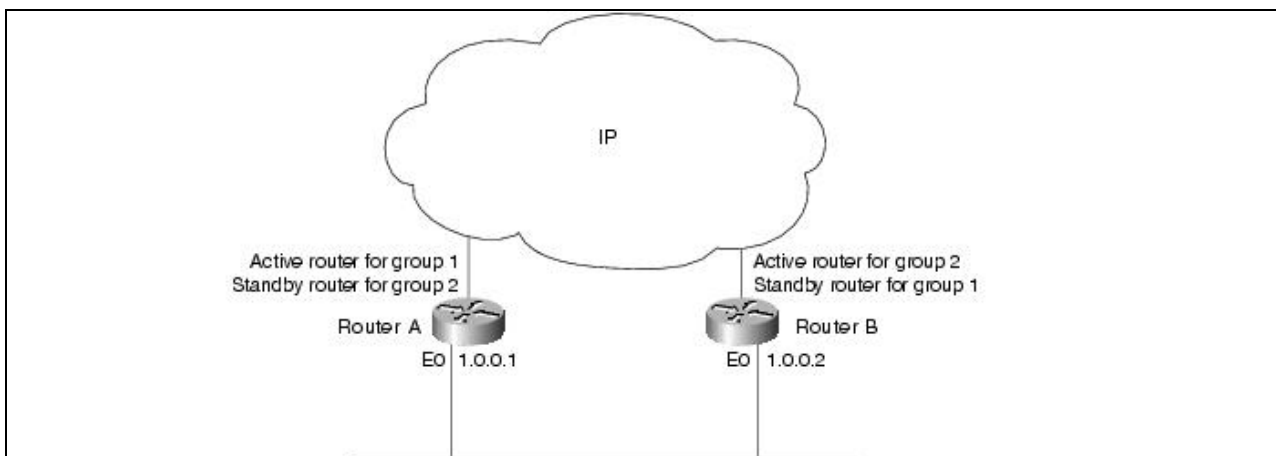
Figure: Load sharing example
