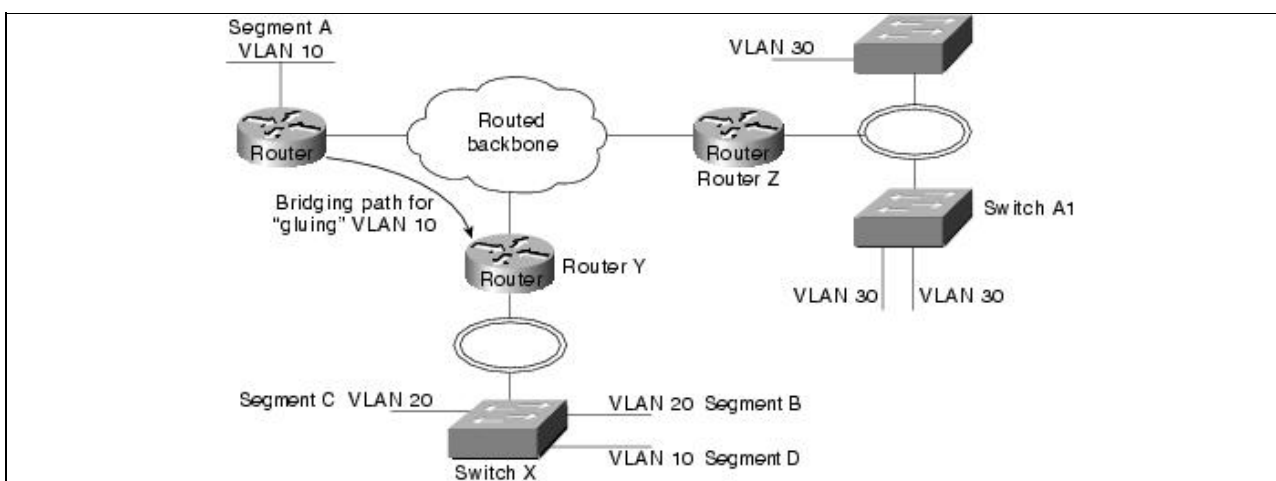
Figure: IEEE 802.10 routed backbone implementation
