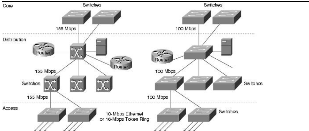
Figure: Large switched/minimal routing design
