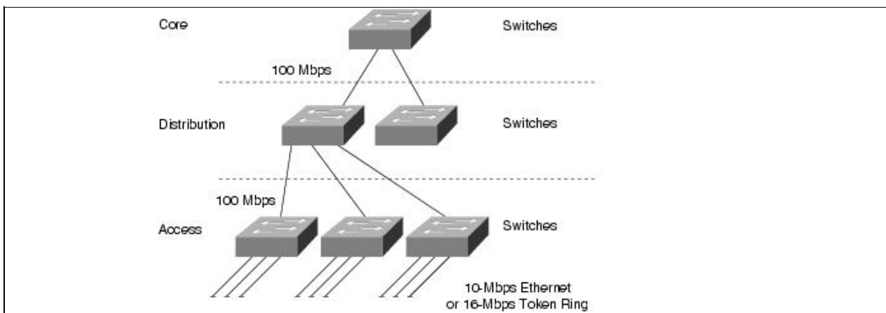
Figure: Scaled switching design
