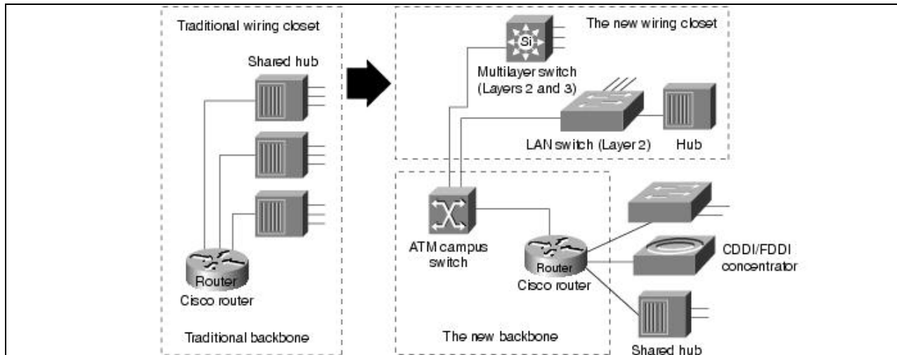
Figure: Evolution from shared to switched internetworks
