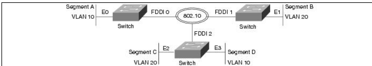
Figure: IEEE 802.10 switched backbone implementation
