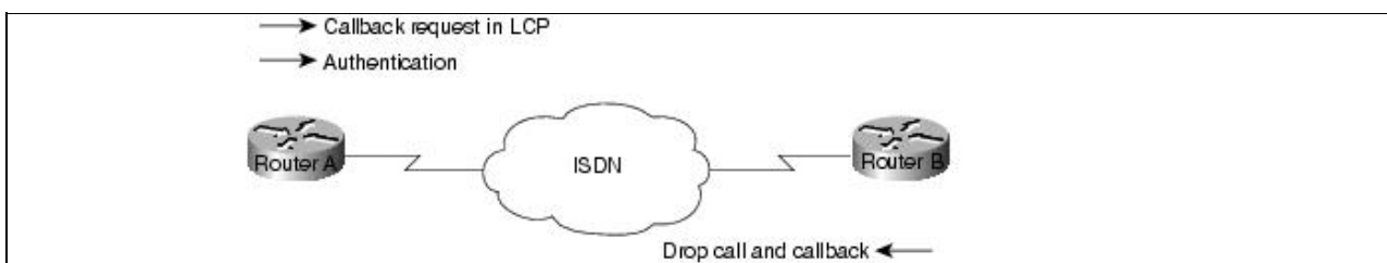
Figure: ISDN callback
