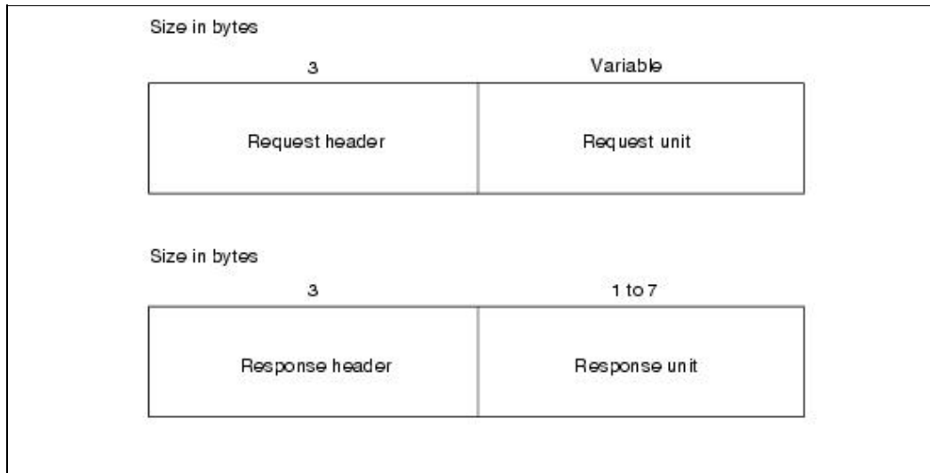
Figure: A Basic Information Unit (BIU) Can Be Either a Request or a Response
