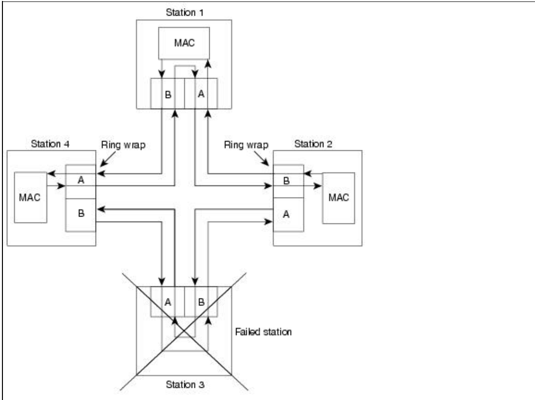
Figure: A Ring also Wraps to Withstand a Cable Failure
