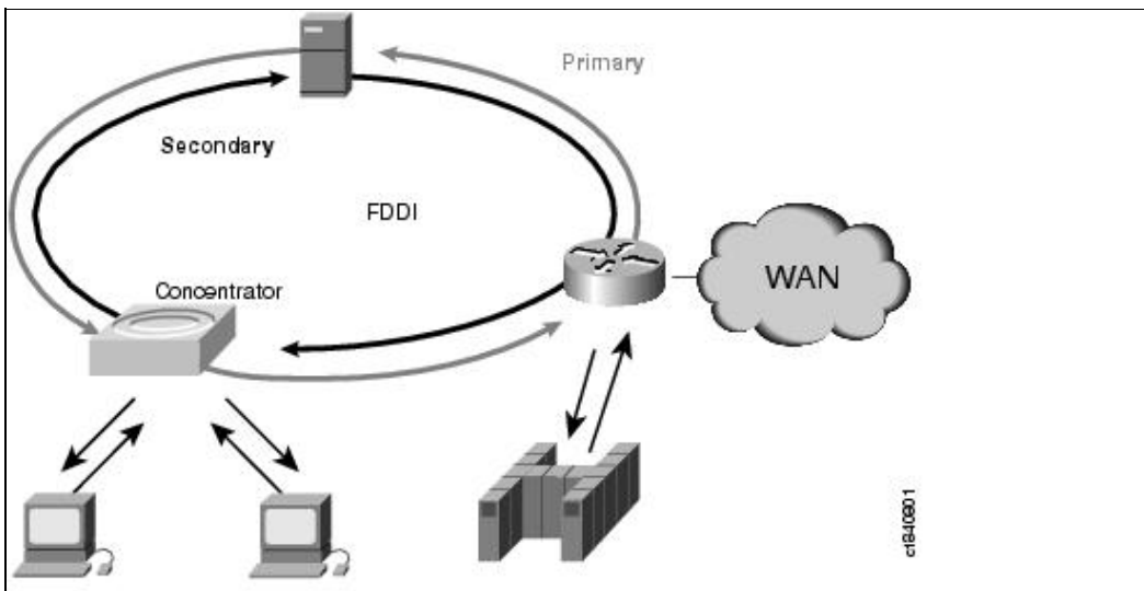
Figure: FDDI Uses Counter-Rotating Primary and Secondary Rings
