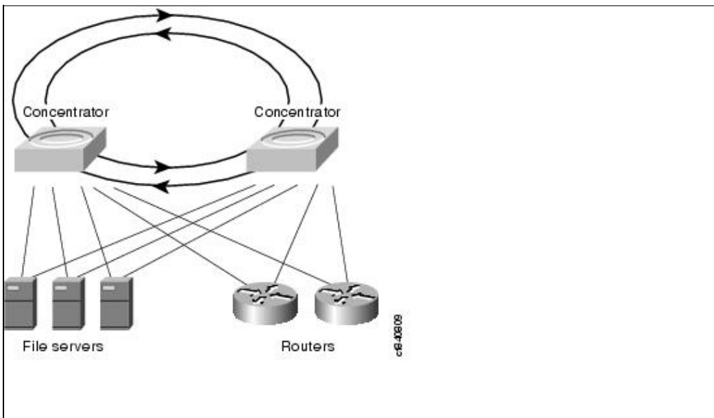
Figure: A Dual-Homed Configuration Guarantees Operation
