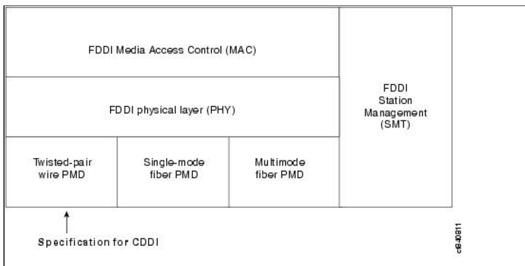
Figure: CDDI TP-PMD and FDDI Specifications Adhere to Different Standards
