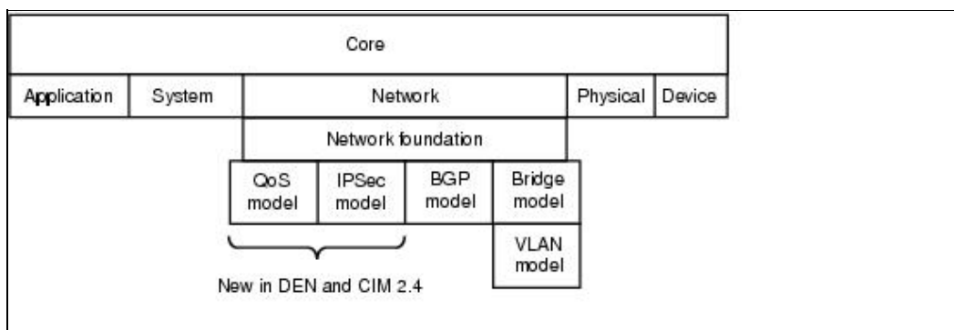
Figure: The CIM Layered Information Model
