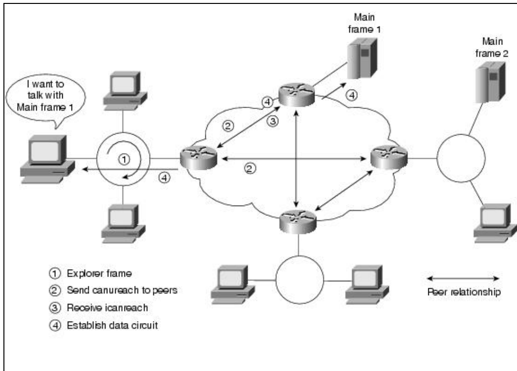
Figure: DLSw Circuit Establishment Flow
