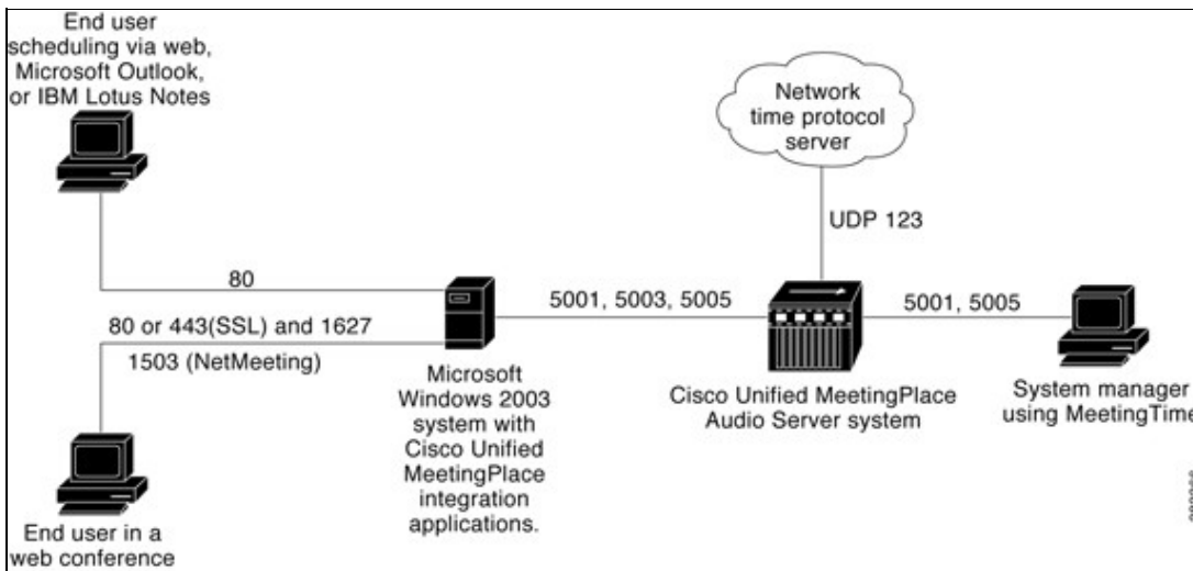
Figure: TCP/UDP Port Requirements
