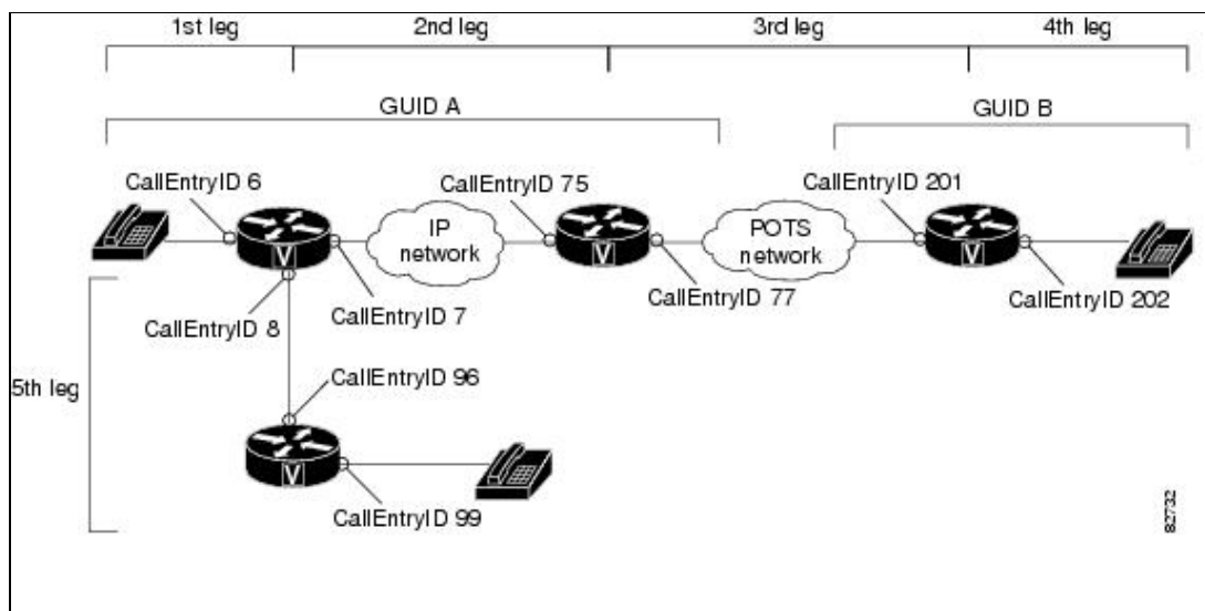
Figure: GUIDs and CallEntry IDs in a Conference Call
