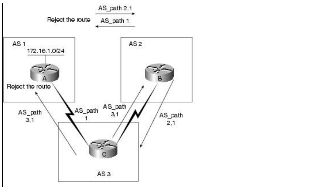
Figure: BGP AS-path Attribute
