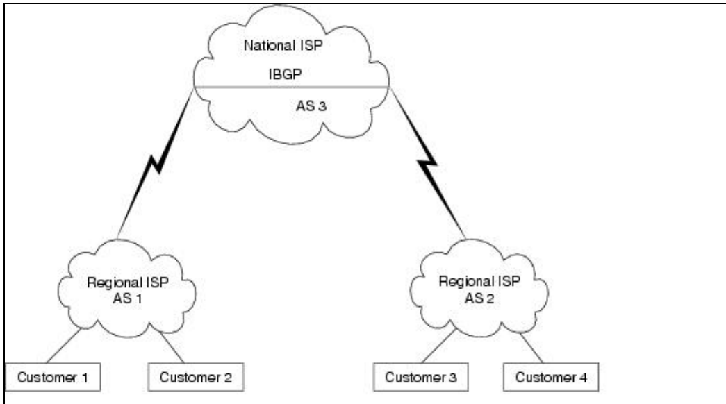
Figure: External and Interior BGP
