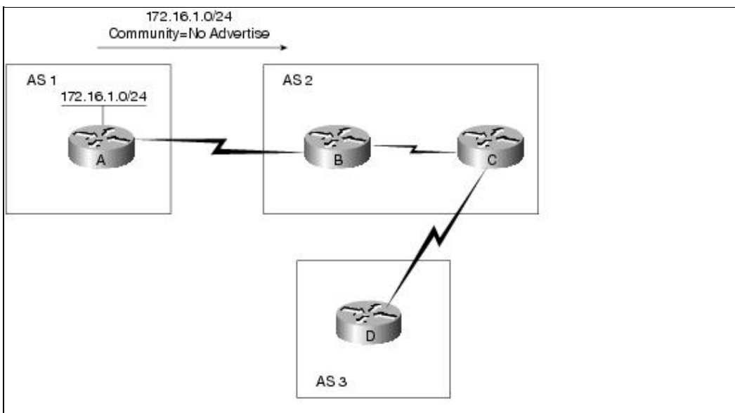
Figure: BGP no-advertise Community Attribute
