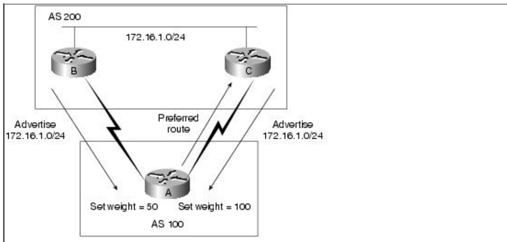
Figure: BGP Weight Attribute
