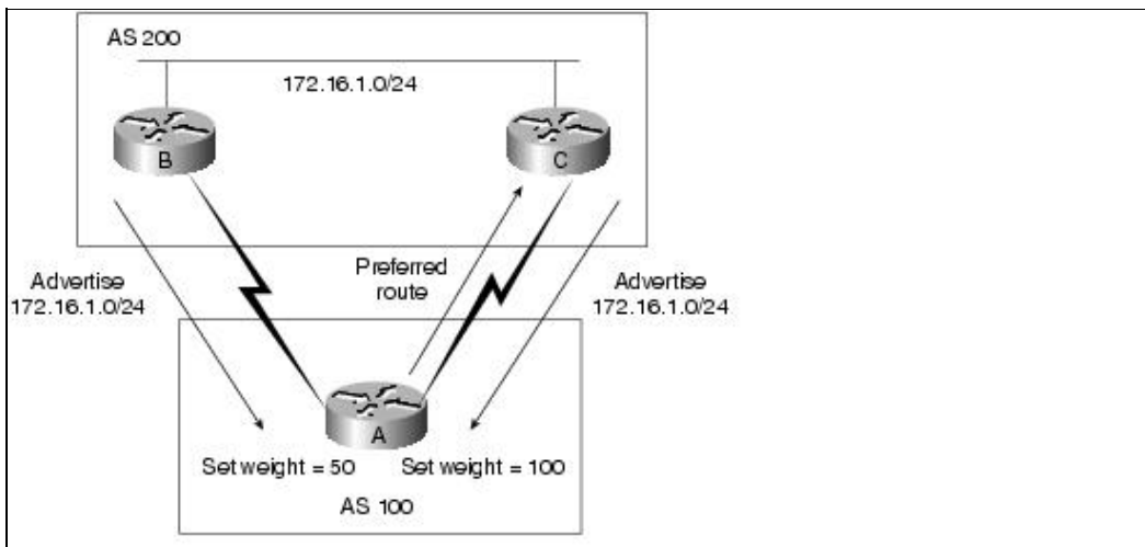
Figure: BGP Weight Attribute
