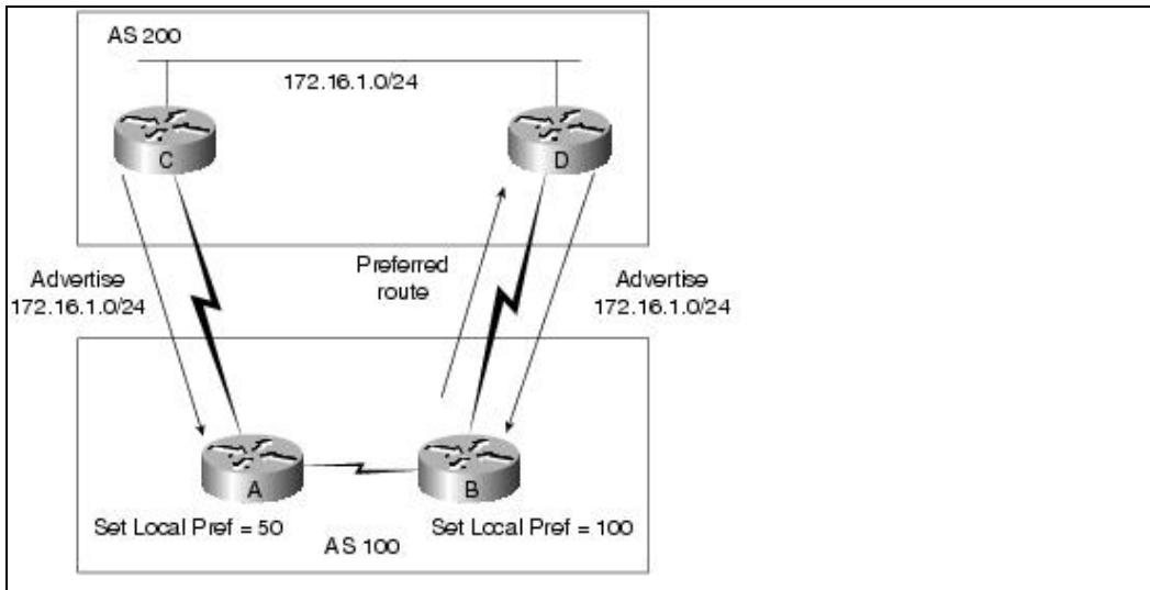
Figure: BGP Local Preference Attribute
