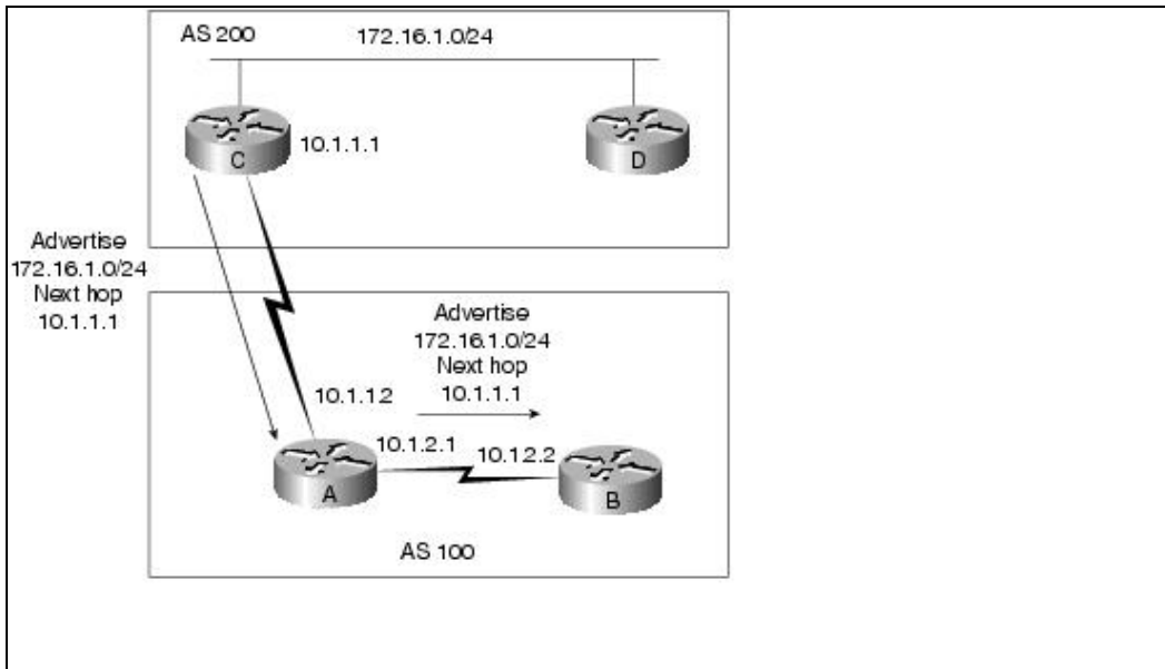
Figure: BGP Next-Hop Attribute
