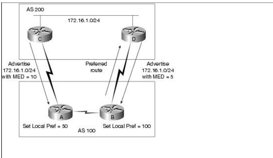
Figure: BGP Multi-Exit Discriminator Attribute
