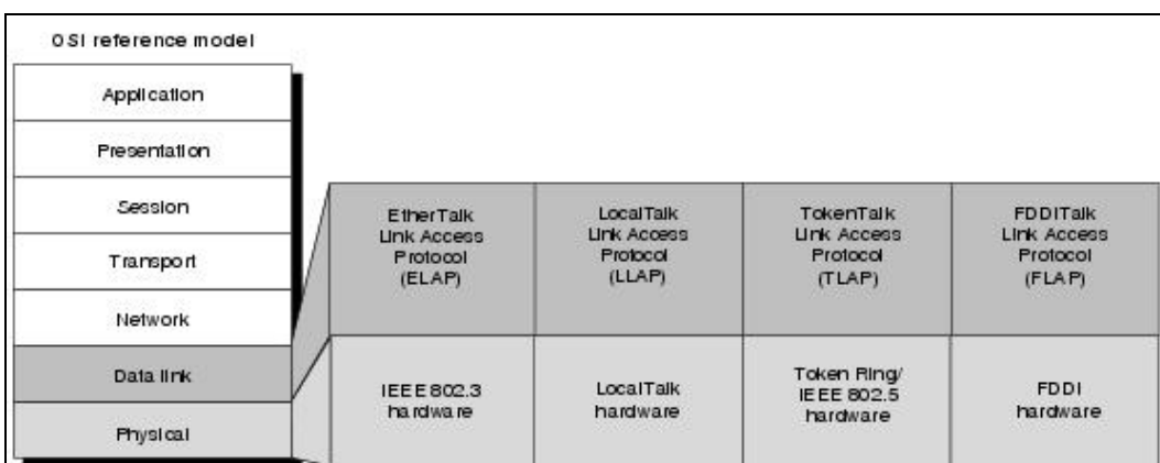
Figure: AppleTalk Media-Access Implementations Map to the Bottom Two Layers of the OSI Reference Model
